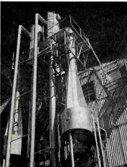
Evaporators like this make possible production of concentrated citrus juices.
